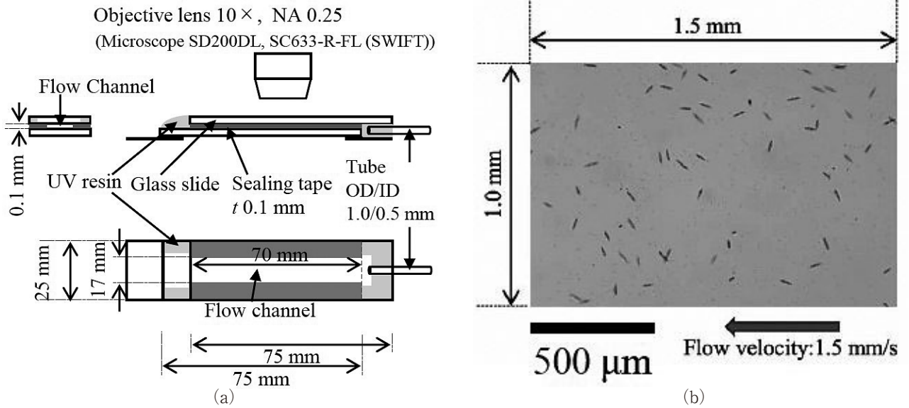
Fig. 1 Schematic diagram of the experimental set-up. (a) Schematic diagram of the flow channel. (b) Exemplar microscopic image of the flowing phytoplankton.
