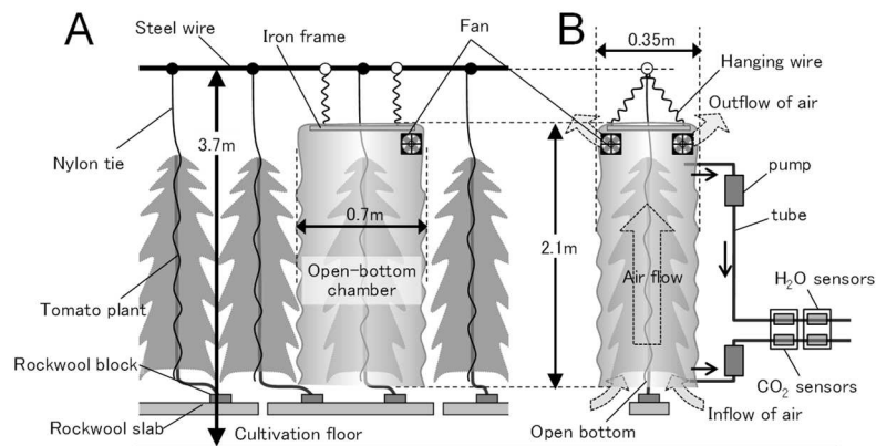
Fig. 1 Schematic diagram of the open-bottom chamber (A: front view, B: side view).
